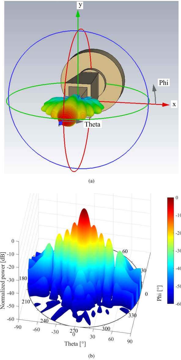
FIGURE 9. 3D representation of the 2D far-field pattern calculated from the measured 2D near-field distribution. (a) Far-field pattern with the antenna CAD data, and (b) representation in a Cylindrical coordinate system.
