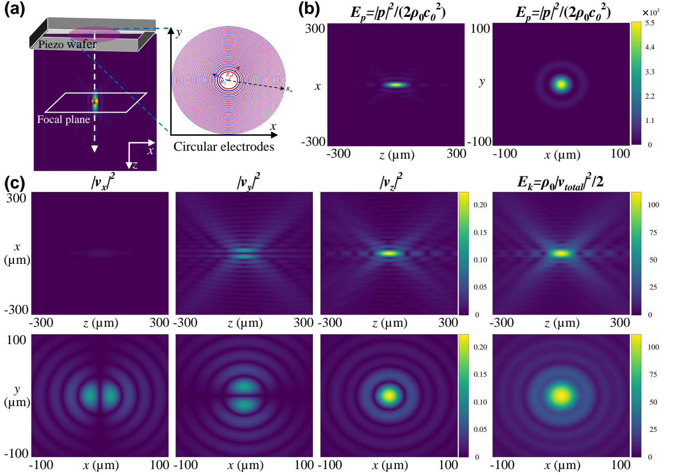
FIG. 2. (a) Schematic of a focused beam of finite aperture 60^\circ synthesized by a binary phase hologram representing the signal that would be generated by circular InterDigitated Transducers. The shape of the circular electrodes are given in the enlarged figure with the designed principle given in Sec. II. (b) The acoustic potential energy E_p = |p|^2 / (2\rho_0 c_0^2) in (x, y = 0, z) and (x, y, z = 0) planes. The pressure amplitude in the source plane is 0.1 MPa for all the simulations. (c) The square amplitudes of the three components of the acoustic velocity |\mathbf{v}_{x,y,z}|^2 and the kinetic energy E_k = \rho_0 |\mathbf{v}_{total}|^2 / 2 are depicted in (x, y, z = 0) plane in the upper row, and in the (x, y = 0, z) plane in the lower row. The information are helpful to understand the trapping properties of Rayleigh particles (size much smaller than the wavelength) in 3D.
