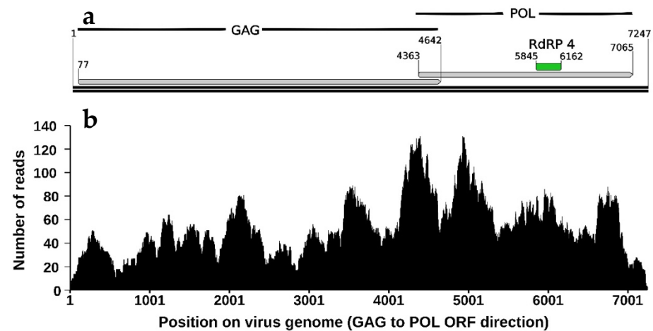
Figure 2. Annotation of HiTV1 genome sequence (a) and read coverage (b). (a) Numbers represent the nucleotide position, and two long horizontal black lines represent the double-stranded RNA sequence. A conserved RdRP 4-like domain (E-value of 1.46 \times 10^{-4} , PF02123) was annotated in green. (b) Using Bowtie2 [60] and SAMtools [61], raw sequence reads from the transcriptome SRR14339788 were mapped onto the HiTV1 contig 1, which resulted from a SPAdes assembly of SRR14339788 reads. The average coverage of the reads across the contig without gaps was 53.79x.
