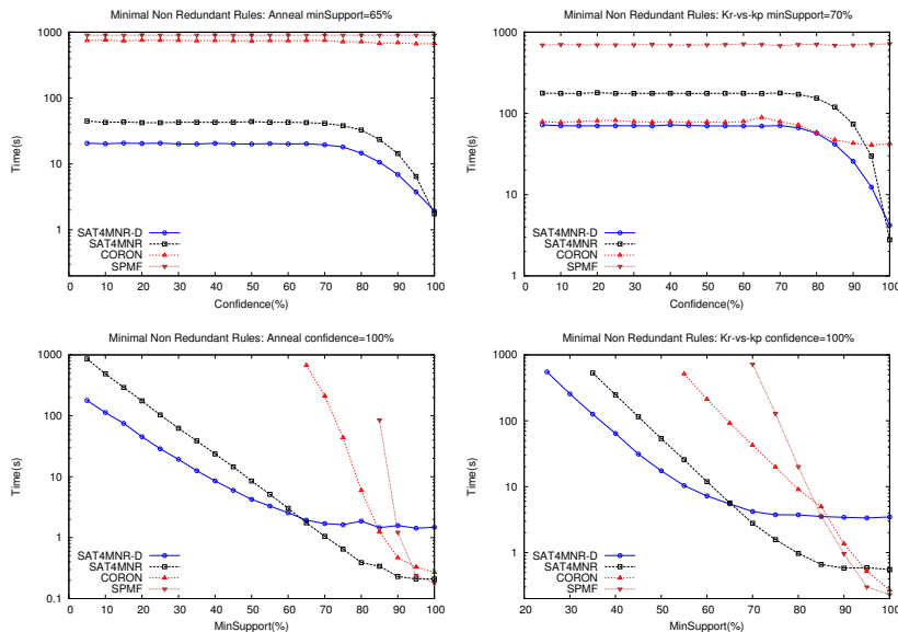
Fig. 1. Results highlights: Annel and kr-vs-kp
