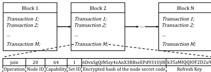
Fig. 4: Example of a blockchain transaction.
