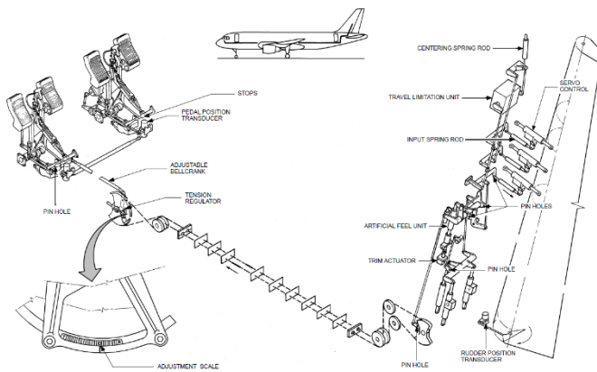
Figure 2. The Airbus A320 yaw control (left: representation centered on mechanical linkages [Lufthansa 1997], right: representation centered on flight controls [BAETC 2008]).
