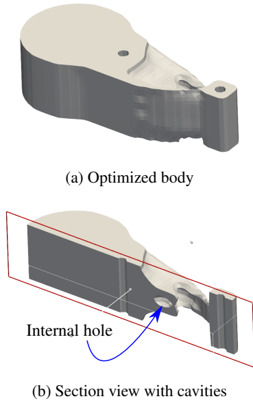
Fig. 15: Cavities in an optimized body
