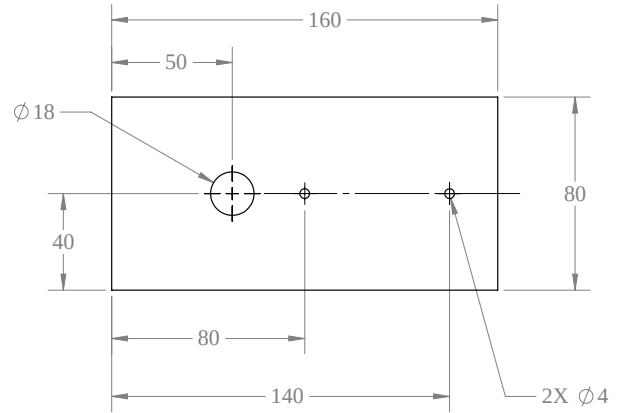
Fig. 7: Initial design domain of bodies \mathcal{B}_1 and \mathcal{B}_3 when the cylinder is included. All dimensions are in millimeters
