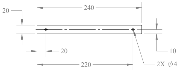
(b) Initial design domain of body \mathcal{B}_2
