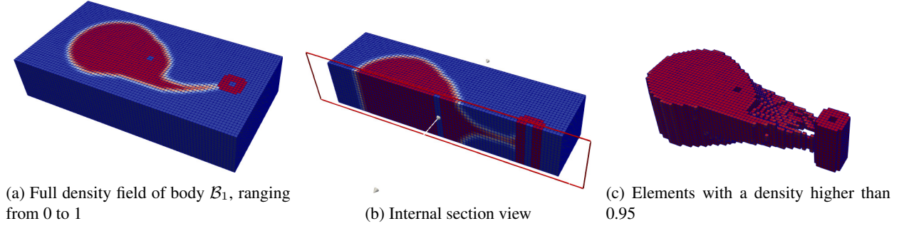
Fig. 10: Voxel-based results of body \mathcal{B}_1 for Case I
