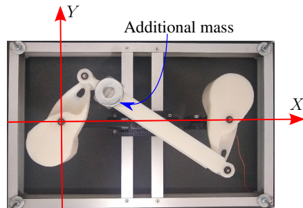
(b) Four-bar linkage with additional mass
