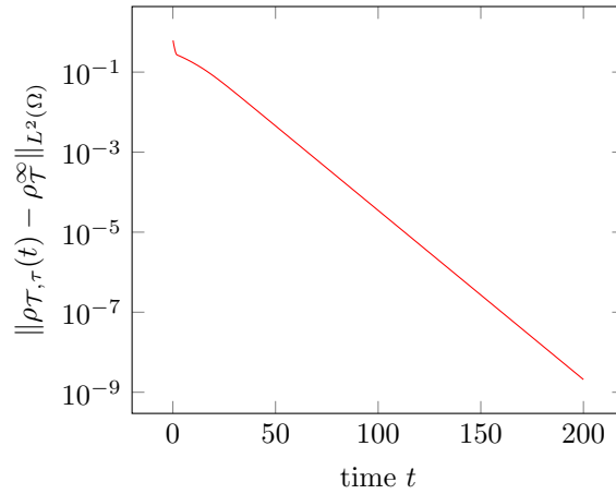
FIGURE 6. Evolution of the L^2 -distance between \rho_{\mathcal{T},\tau}(t, \cdot) and \rho_{\mathcal{T}}^{\infty} as a function of t – non-equilibrium case (76).
