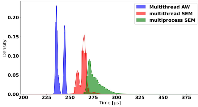
Figure 8 Normalized histograms with their estimated probability density function of a pipeline composed of one MVM unit with various synchronization approaches (SEMAaphore and Active Wait) over 1M iterations on the Jetson Xavier
