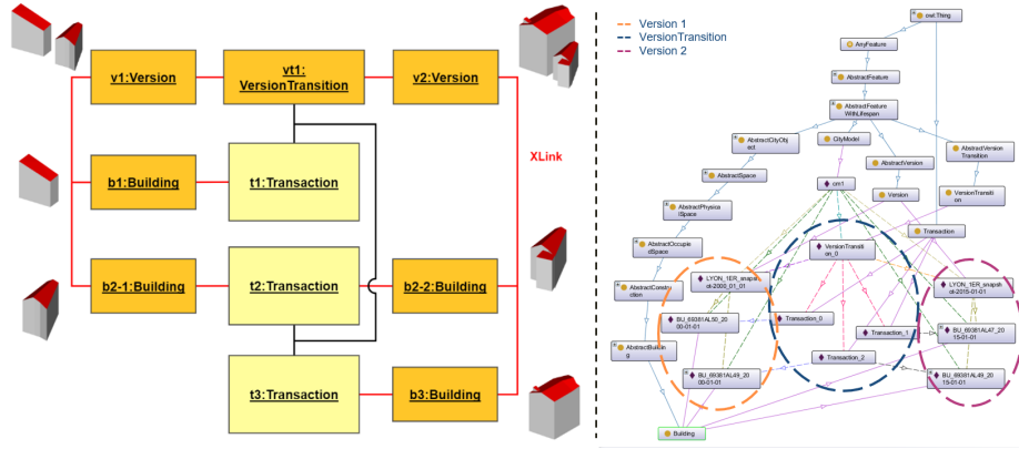
Fig. 2. 3 building historical successions based on the CityGML 3.0 Versioning module; Version graph overview 7 (left); Ontograp visualization of generated RDF graph produced by UD-Graph [26] (right)
