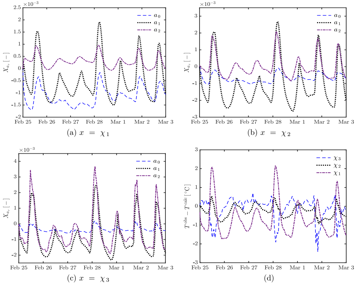
Figure 6. Variation of the calculated sensitivity coefficients for (a) first, (b) second and (c) third sensor locations; (d) residuals between the calculated and the measurements.
