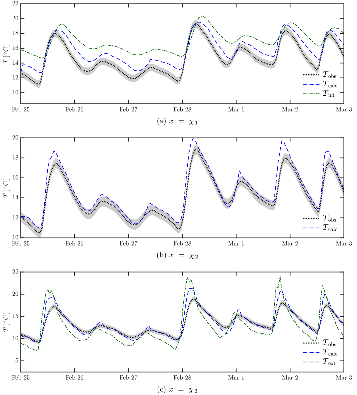
Figure 3. Variation of the observations and computed temperature using a priori material properties, without effect of the moisture content, for (a) the first sensor and the interior wall surface; (b) the second sensor position; (c) the third sensor and the exterior wall surface.
