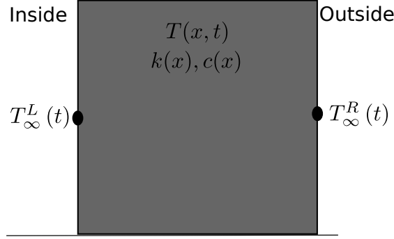
Figure 1. Illustration of a wall domain.
