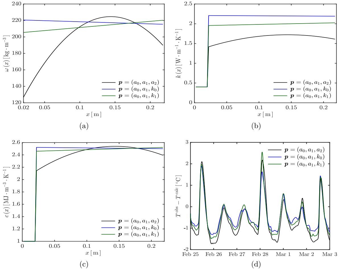
Figure 5. Variation of the (a) the estimated moisture distribution representation in the brick layer, (b) estimated thermal conductivity and (c) volumetric heat capacity representations; (d) the difference between the observations and the calculated temperature values for different estimates at the first sensor location.
