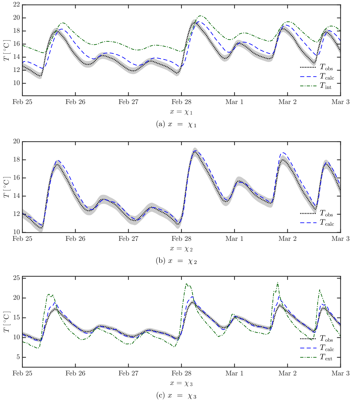
Figure 4. Variation of the observations and computed temperature using the estimated moisture content distribution, for (a) the first sensor and the interior wall surface; (b) the second sensor position; (c) the third sensor and the exterior wall surface.
