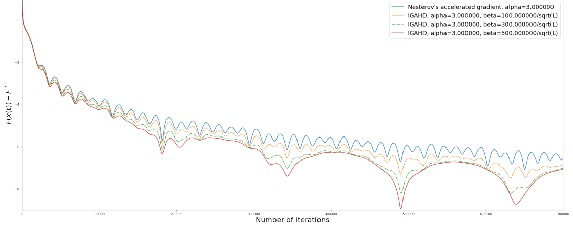
Figure 1: Convergence rate of IGADH for several values of \beta for a least squares problem ( N = 500 ).
