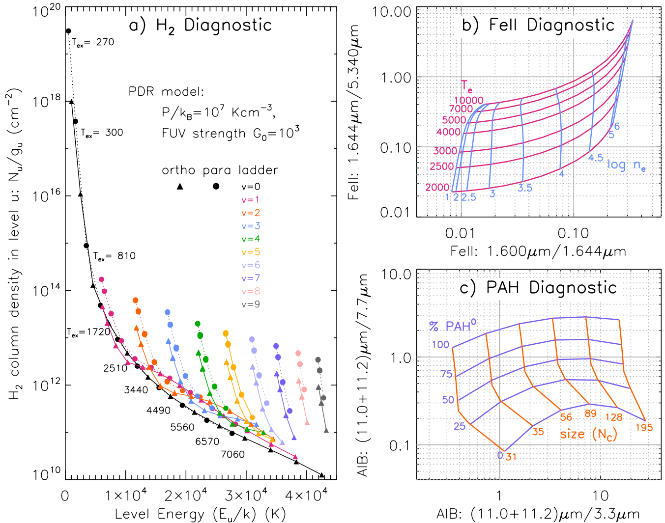
Figure 4. Example IR PDR diagnostics: a) Excitation diagram from H 2 lines in PDRs, that are observable by MIRI and NIRSpect, as a tracer of the warm and hot (UV-pumped) excitation temperatures (excitation temperatures derived from the level populations by a local Boltzmann fit are indicated); b) The [Fe II] lines as a tracer of the temperature and density distribution from the ionized gas to the PDR (Dere et al. 2019); c) AIB emission ratios as a tracer of PAH size (in function of number of carbon atoms, N_C ) and charge (in function of the neutral PAHs fraction, i.e. \text{PAH}^0/(\text{PAH}^0+\text{PAH}^1) ), computed from harmonic IR spectra using PAHdb and assuming an interstellar radiation field (see Section 8 for a description of PAHdb). Figure adapted from Maragoudakis et al. (2020).
