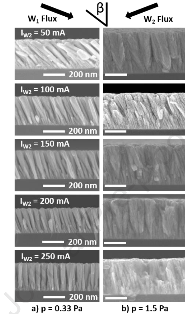
Fig. 3: Cross-section scanning electron microscopy observations of W thin films deposited at a) low pressure and b) high pressure with a constant target current ( I_{W1} = 140 mA) and various I_{W2} target currents.
