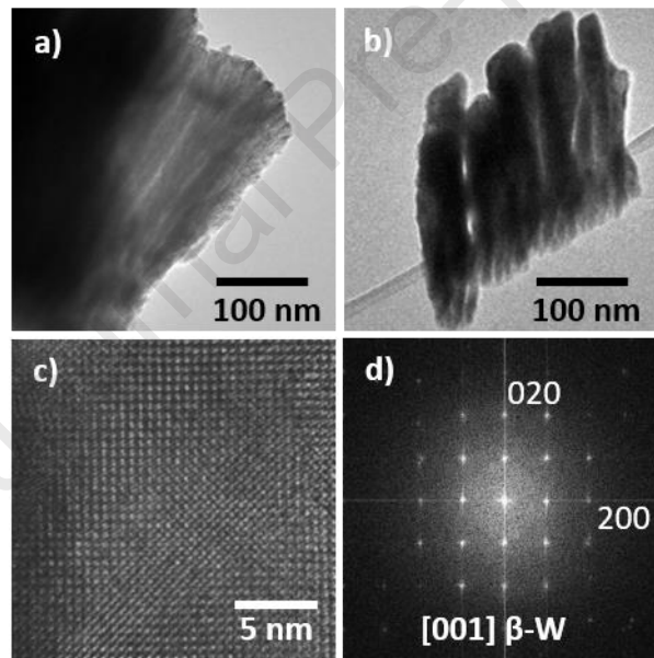
Fig. 6: TEM images of columnar W thin films deposited at a) high pressure and b) low pressure with IW_2 = 200 \text{ mA} . c) HRTEM image of a crystallized area acquired for the sample grown at low pressure and d) its fast Fourier transform (FFT) pattern corresponding to [001] zone axis of \beta -W.
