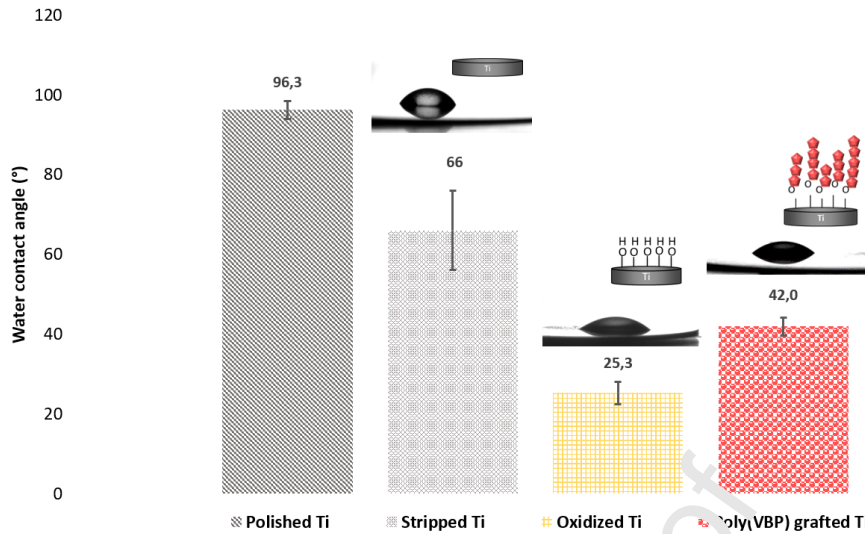
Fig. 7. Water contact angle measurements on polished Ti, stripped Ti, oxidized and poly(VBP) grafted Ti.
