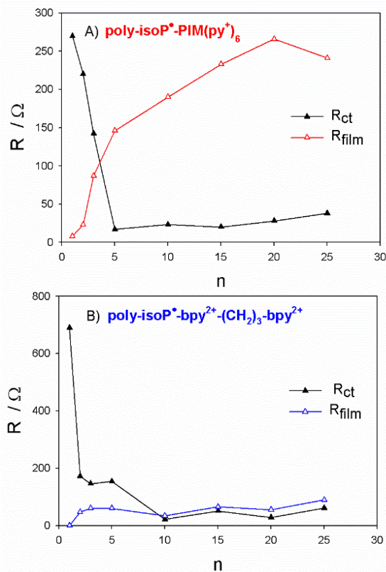
Figure 8. Plot of the R_{ct} and R_{film} of the thin films versus n (number of iterative scan, \nu = 100 \text{ mV s}^{-1} , between -1.1 V and +0.9 V). A) poly-ZnT 2 isoP•-PIM(py + ) 6 , B) poly-ZnT 2 isoP•-bpy 2+ -(CH 2 ) 3 -bpy 2+ .
