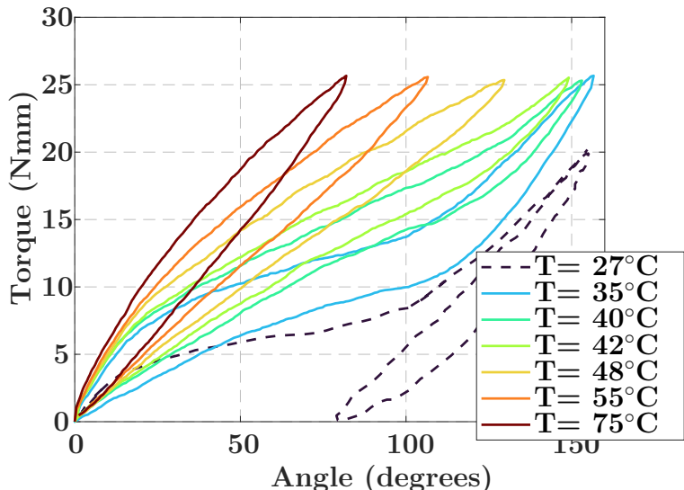
Figure 5: The isotherm test results: Torsion test of two 0.5mm diameter and 5.4mm length wires undergoing five cycles at seven temperatures. Ramp form loading/unloading torque with a maximum value of 26Nmm is cyclically applied at a rotation rate of 3 degree/s.
