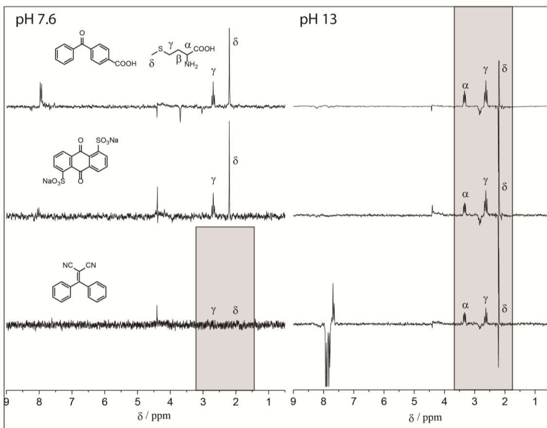
Figure 1 ^1\text{H} -CIDNP spectra obtained upon photooxidation of 1 with B (top), AS (middle) and CN (bottom) a) at pH 7.6 and b) pH 13. All spectra are recorded 1 \mu\text{s} after the laser flash (355 nm, 8 ns and correspond to those shown in [33], 100 \mu\text{s} after the laser pulse)
