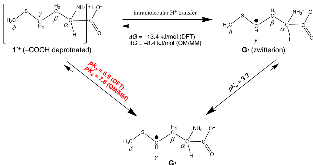
Scheme 3. Thermodynamic cycle for calculating the pK_a value for the deprotonation of \mathbf{1}^{*+} to yield \mathbf{G}\cdot .
