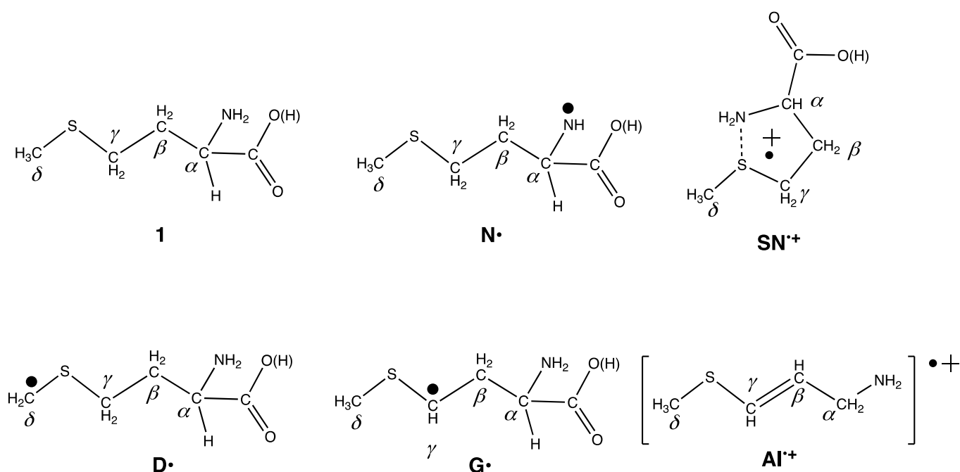
Scheme 1: Radicals based on 1 discussed in this manuscript (differently charged protonated, deprotonated, zwitterionic forms are omitted for clarity, accordingly, we have placed the hydrogen at the carboxyl group in brackets).
