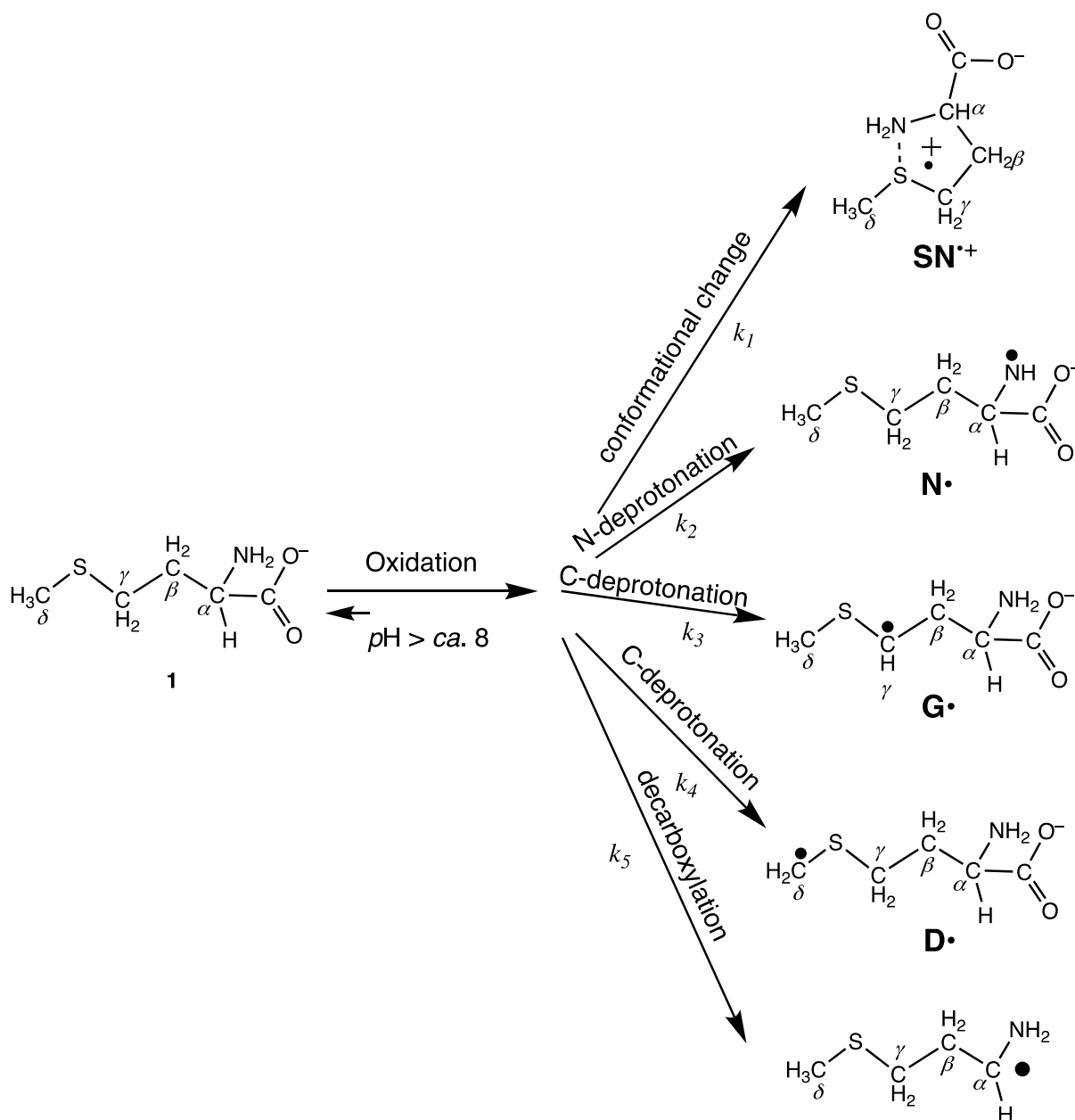
Scheme 4. Radicals involved in primary processes (ns- \mu s time scale) upon the oxidation of 1 under basic conditions (for better comparison the negative charges are omitted from the acronyms of the radicals).
