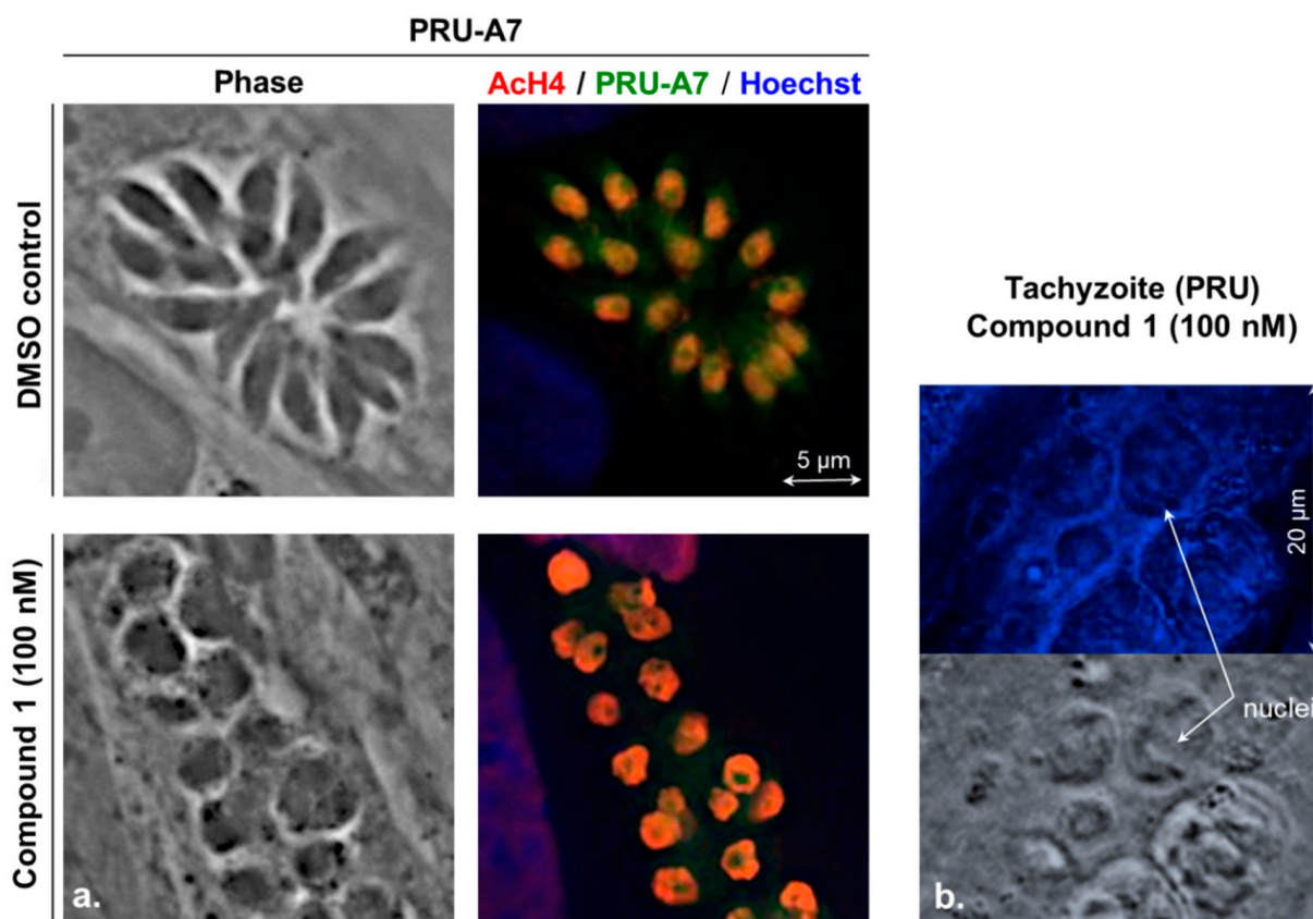
Figure 5. (a) In vitro tachyzoites PRU- \Delta hxgprt-A7 strain (PRU-A7) treated with the compound 1 results in an increased level of histone-H4 acetylation (AchH4) associated with dysmorphic features (increased size, giant polynucleated parasites, rounded shape); Fixed cells, AchH4 in red (anti-acetyl-H4 polyclonal rabbit antibodies (primary antibodies) (Millipore), followed by the secondary antibodies goat anti-rabbit IgG coupled with either Alexa Fluor 568 (Invitrogen) at a 1:1000 dilution), tachyzoite GFP protein (PRU-A7 in green), HFF, and tachyzoite DNA in blue (Hoechst) (b) Localization of the compound 1 in treated PRU tachyzoites observed by microscopy (c = 100 nM, 48 h, exposure time 1000 ms).
