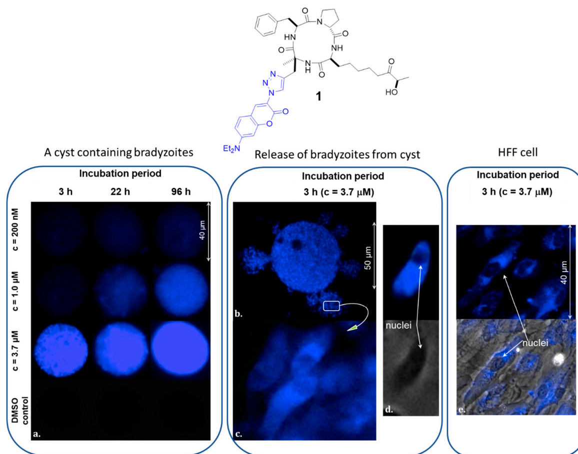
Figure 3. (a) Ex vivo T. gondii cysts incubated with compound 1 at a growing concentration (c = 200 nM to 3.7 μM) for 3, 22 and 96 h, 37 °C, exposure time = 100 ms; (b) Cyst treated with 1 (c = 3.7 μM for 3 h and released from the cyst, 37 °C, exposure time = 100 ms; (c,d) Bradyzoites at a higher magnification ( \times 100 ); (e) HFF cells treated with 1 (exposure time = 100 ms).
