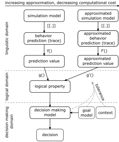
Fig. 6. Conceptual framework.
