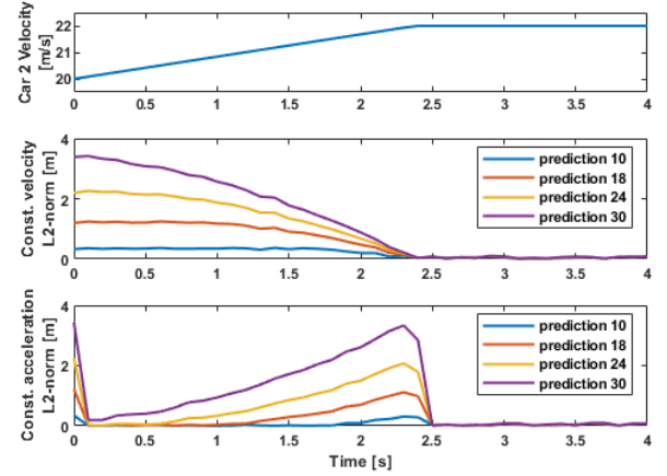
Fig. 4. Car 2's velocity profile, compared with the L2 errors made by the constant velocity and acceleration prediction models.
