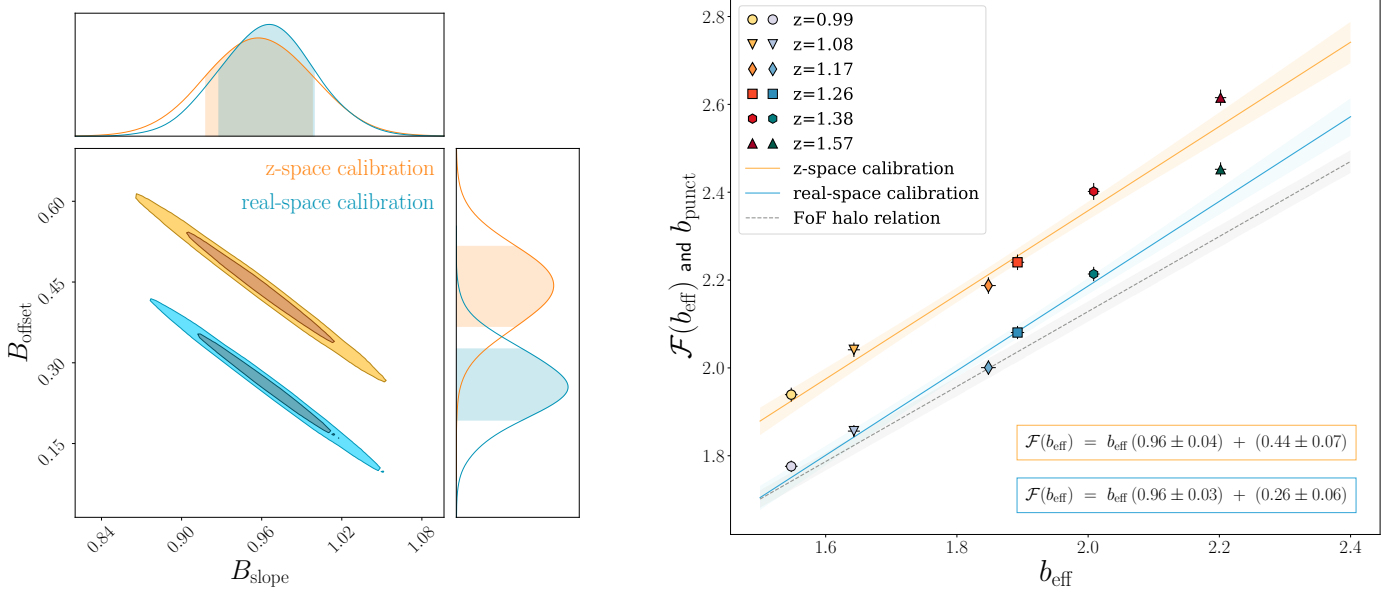
Fig. 2. Calibration of the relation \mathcal{F}(b_{\text{eff}}) from Eq. (9), required for the conversion of the threshold \delta_{\text{vir}} in Eq. (7). Left: the 68% and 95% confidence levels in the B_{\text{slope}}-B_{\text{offset}} plane for the void catalogues built both in real (blue) and in redshift space (orange). Right: the solid lines represent the resulting linear relations \mathcal{F}(b_{\text{eff}}) obtained with the calibrated coefficients B_{\text{slope}} and B_{\text{offset}} for real (blue) and redshift space (orange), while the shaded regions indicate an uncertainty of 2\sigma on the relationships. The markers represent the calibration obtained for each bin of redshift, leaving b_{\text{punct}} as the only free parameter of the void size function model when fitting the measured void number counts. This alternative calibration provides a value of b_{\text{punct}} for each redshift of the sample and is associated with the value of the effective bias b_{\text{eff}} of the Flagship galaxies at that specific redshift. As a comparison we also show the linear function calibrated using FoF dark matter haloes in real space by Contarini et al. (2019), displayed with a dashed grey line.
