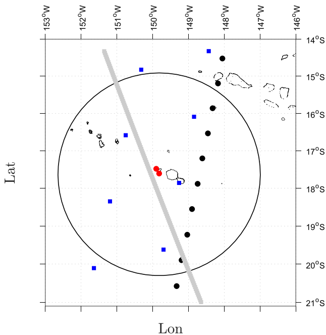
Figure 4. Map centered on the Island of Moorea (wave gauges location in red). The black thin circle line indicates a 300 km distance from Moorea. Black dots: mean position of the Surface Waves Investigation and Monitoring L2 products on 06 May 2019 between 16:49:29 and 16:51:06. Blue squares: position of the Synthetic Aperture Radar S1 imageries on the same day between 15:35:32 and 15:37:44. In gray: ground track of the Jason-3 ku-band radar the same day between 16:22:51 and 16:25:09.
