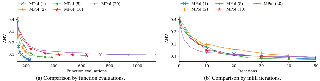
Figure 12 Comparison of Kriging with continuous relaxation and MPoI (Minimum Probability of Improvement) infill criterion for different infill batch sizes. For an infill batch larger than 1, the modulated infill criterion is used (see Fig. 9). In terms of function evaluations, choosing only 1 infill point per iteration results in fastest convergence. If parallel evaluation is possible, infill sizes larger than 1 can result in faster convergence.
