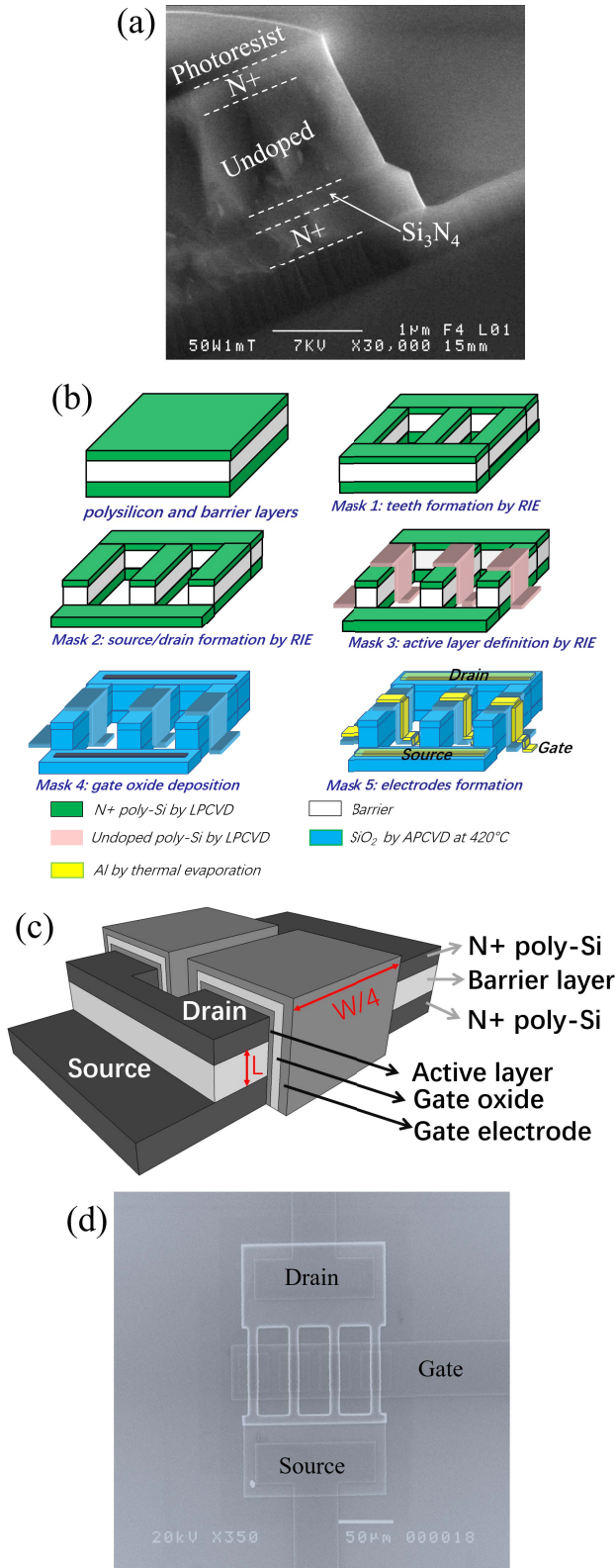
Fig. 1. (a) SEM image of vertical sidewall incorporating Si 3 N 4 barrier layer, (b) five-mask fabrication process of the vertical TFT, (c) three-dimensional configuration of a two-tooth vertical TFT, and (d) SEM image of a four-tooth vertical TFT, where eight channels were formed at the sidewalls.
