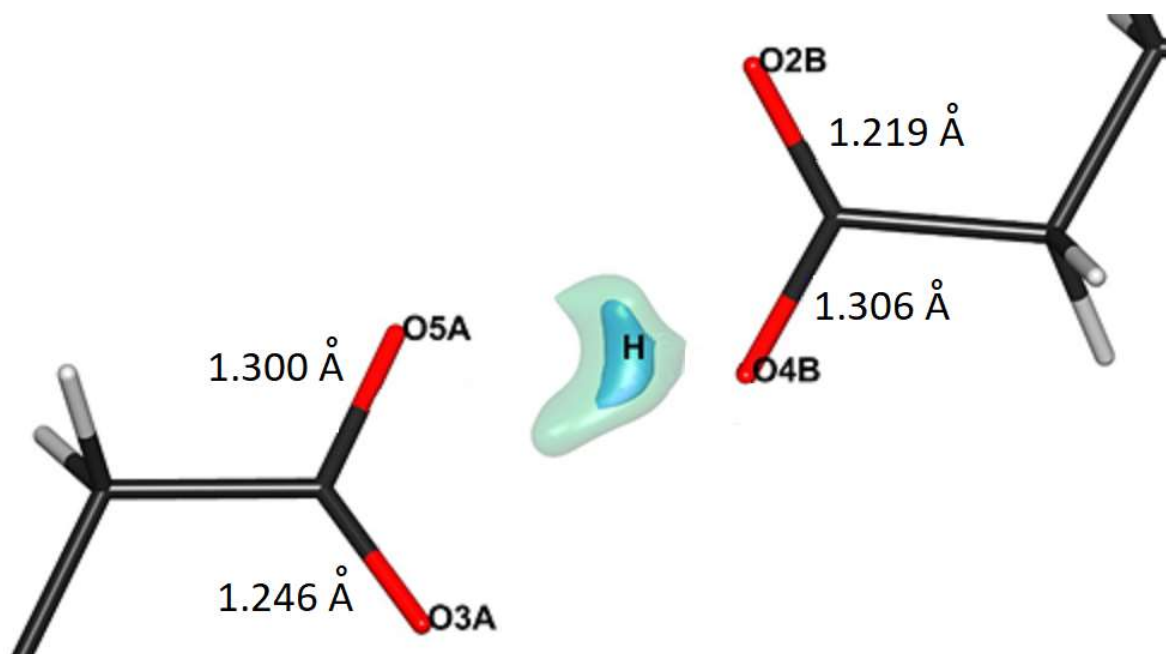
Fig. 2 Fourier residual omit H map in the O4B...O5A region. Contour levels 0.4 (blue) and 0.5 (green) \text{e.}\text{\AA}^{-3}
