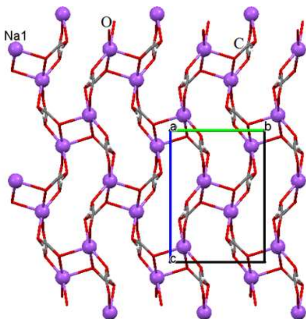
Fig. 5 Projection of a 2-D layers of sodium cations in the crystal structure along the a -axis. The carbon chains of lauric acid and laurate molecules have been omitted for clarity.
