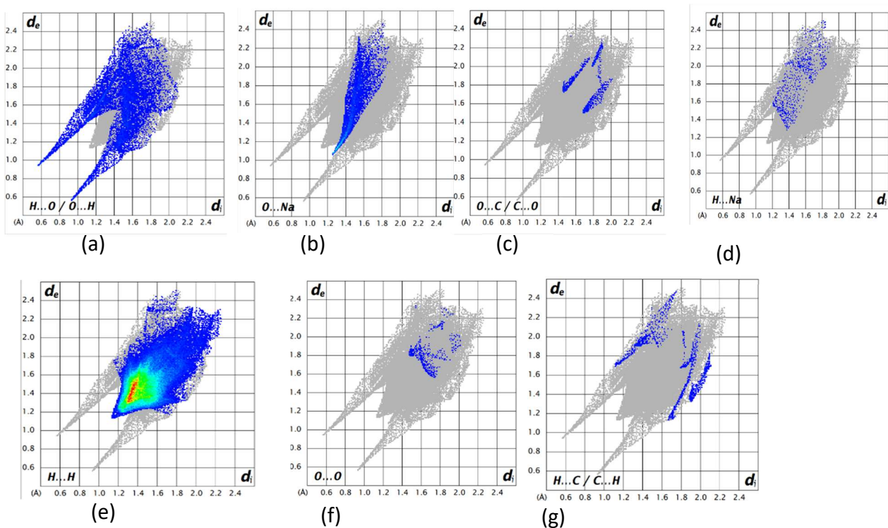
Fig. 9 Fingerprint plots in (d_i, d_e) of the main contacts on the Hirshfeld surface. The graphs were obtained with CrystalExplorer17 program [45].
