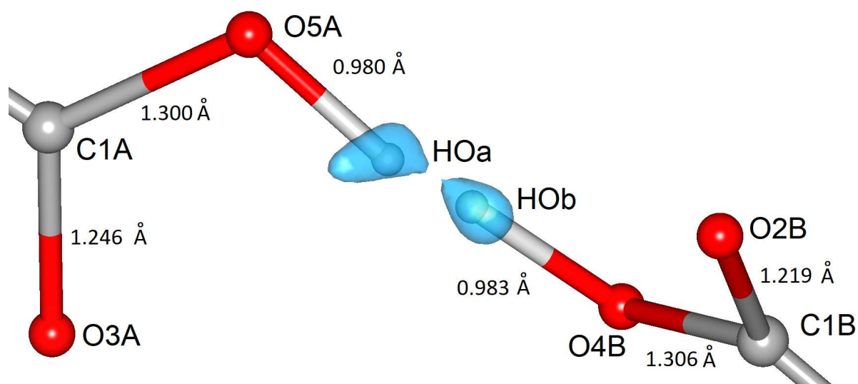
Fig. 3 The omit H map in blue at contour level at 0.27 \text{ e.}\text{\AA}^{-3} . The Fourier residual map using terms (F_{\text{obs}} - F_{\text{calc}}) * R was computed by applying a noise reduction technique.
