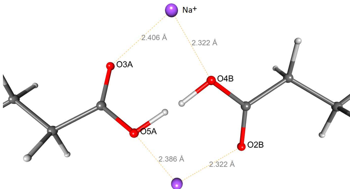
Fig. 6 View of the two closest sodium cations interacting with the oxygen atoms of the title compound.
