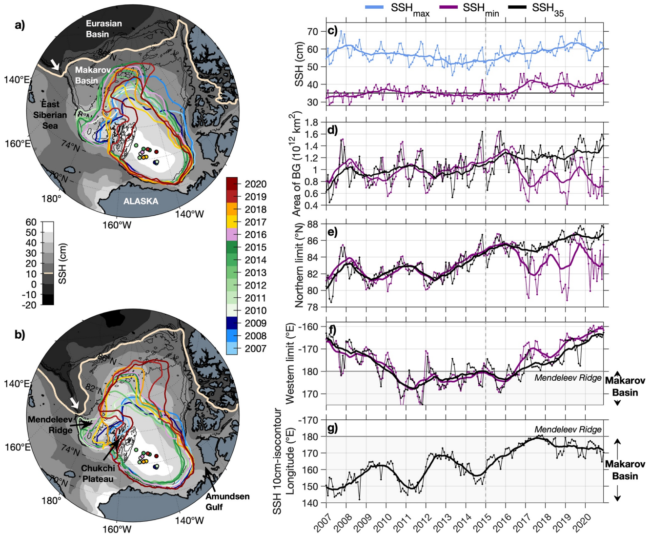
Figure 7. (a) Yearly mean SSH isocontours of the Beaufort Gyre limit from 2007 to 2020 following Regan et al. (2019). Centers of the Beaufort Gyre determined from the location of \text{SSH}_{\text{max}} are indicated for each year. The background color is the SSH field in 2011 and the isocontour \text{SSH} = 10 \text{ cm} is shown in beige. Black isocontours in the background indicate IBCAO bathymetry 2,000, 1,000, and 500 m (thick black line). (b) same as (a) with Beaufort Gyre limit obtained from SSH isocontour 35 cm. Background color is the SSH field in 2016. (c) \text{SSH}_{\text{max}} corresponding to the Beaufort Gyre center (blue) and \text{SSH}_{\text{min}} corresponding to the BG limit in (a) (purple). The black line is for \text{SSH} = 35 \text{ cm} . (d) Area of the Beaufort Gyre computed in Figures 11a (purple) or 11b (black). (e) Northern limit ( ^{\circ}\text{N} ) of the Beaufort Gyre using \text{SSH}_{\text{min}} (purple) or 35 cm SSH isocontour (black). (f) Western limit ( ^{\circ}\text{E} ) of the Beaufort Gyre using \text{SSH}_{\text{min}} (purple) or 35 cm SSH isocontour (black). (g) Longitude of the easternmost point of SSH 10 cm isocontour indicated by the white arrow on (a and b). From (c) to (g), thin lines are monthly means and thick lines are for 12-month running mean.
