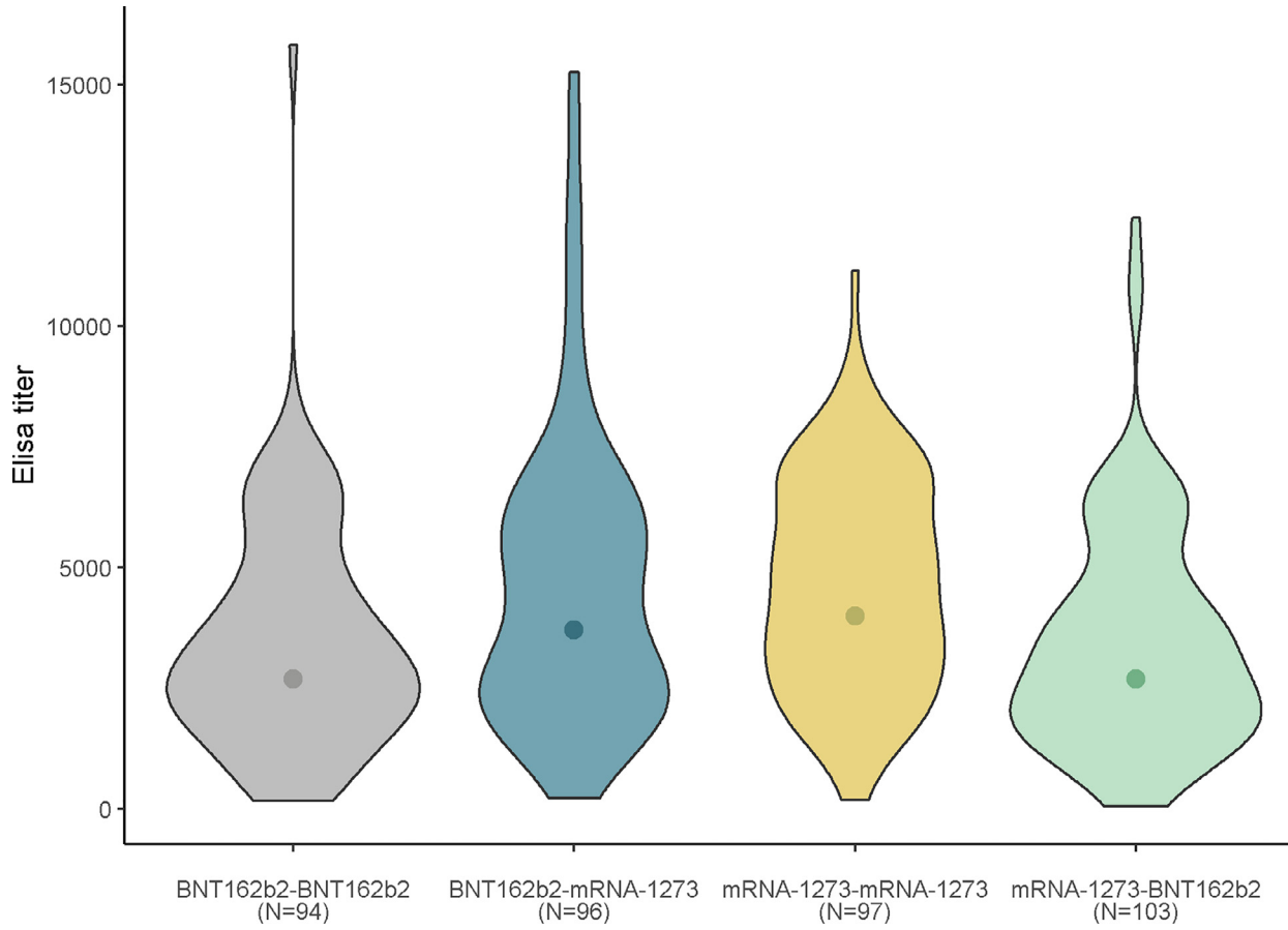
Figure 2. Violin plots of anti-spike antibody titers determined by Elisa 28 days post dose 2 of vaccine. Legend: Within each diagram, the geometric mean is represented by a point.
