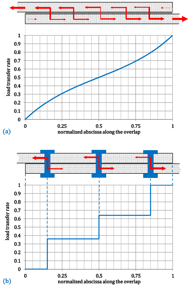
Fig. 2. Load transfer in a single-lap bonded (a) joint (a) and in a single-lap bolted joint (b).
