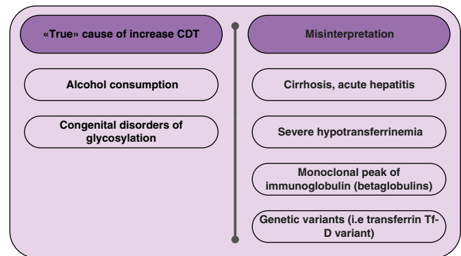
Fig. 1. Comprehensive causes of CDT increase. CDT, carbohydrate deficient transferrin.
