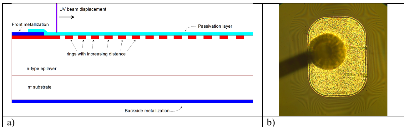
Fig. 2. a) Schematic cross section view of half vertical PiN diodes protected by 22 field rings (principle is sketched here only with 13 rings), b) photograph of the diode with the 50 \mu\text{m} (diameter) gold ball bonding
