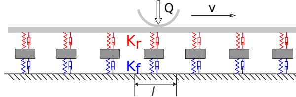
Figure 1: Model of the periodically supported beam.
