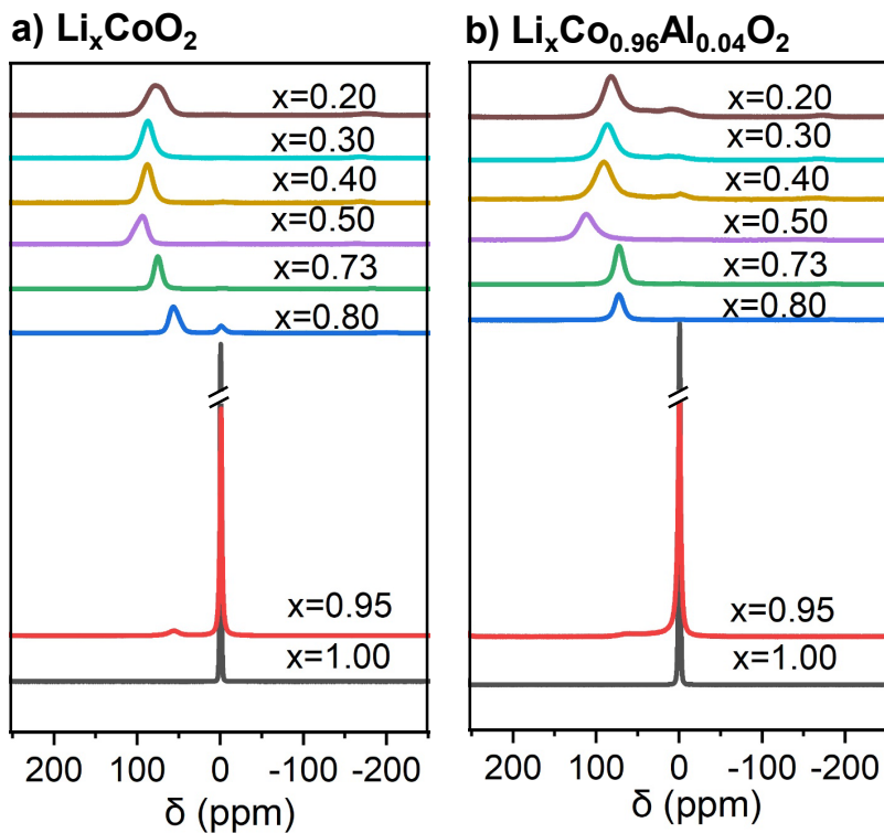
Figure 3: Ex-situ {}^7\text{Li} MAS NMR spectra for a) \text{Li}_x\text{CoO}_2 and b) \text{Li}_x\text{Co}_{0.96}\text{Al}_{0.04}\text{O}_2 recorded using a rotor-synchronized Hahn echo sequence ( \nu_R = 30 kHz). Arbitrary intensities are used here to better visualize the shifts.
