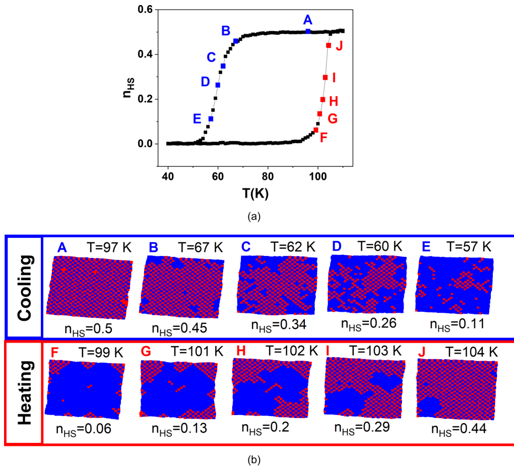
FIG. 10. (a) Reverse-LITH of the HS fraction, n_{\text{HS}} , obtained by MC simulations under a permanent irradiation for W^{\text{opt}} = 2 \times 10^{-3} (a.u.). The simulations are done by cooling from the antiferromagnetic metastable configuration at n_{\text{HS}} = 0.5 at T = 110 K until 40 K and then heating back. (b) Selected snapshots showing the spin organization along the process. Red and blue dots correspond to HS and LS sites. All other parameters are the same as those of Fig. 8.
