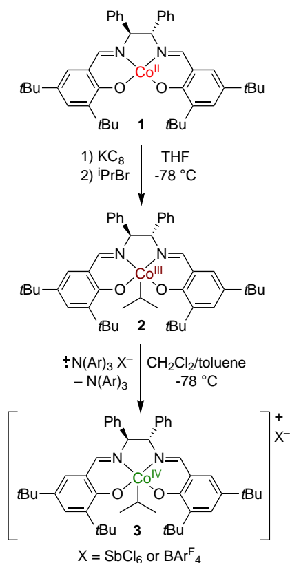
Scheme 2. Preparation of (salen Ph )Co( i Pr) + ( 3 ).
