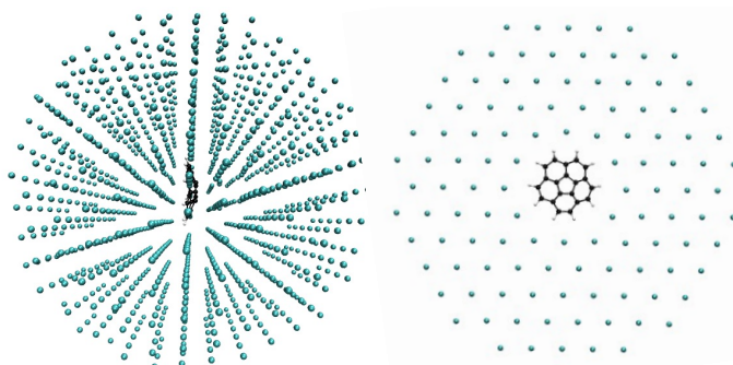
Figure 2. Optimised structure of \text{C}_{20}\text{H}_{10} :Ar obtained at the DFTB/FF level of theory. The total system is reported on the left hand side, the selection of the [111] plane where corannulene is inserted is represented on the right hand side.
