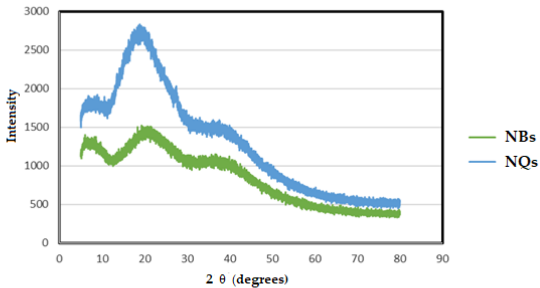
Figure 9. X-ray diffraction (XRD). Pattern of inulin non-charged nanoparticles (NBs) (green line) and inulin nanoparticles loaded with quercetin (NQs) (blue line).
