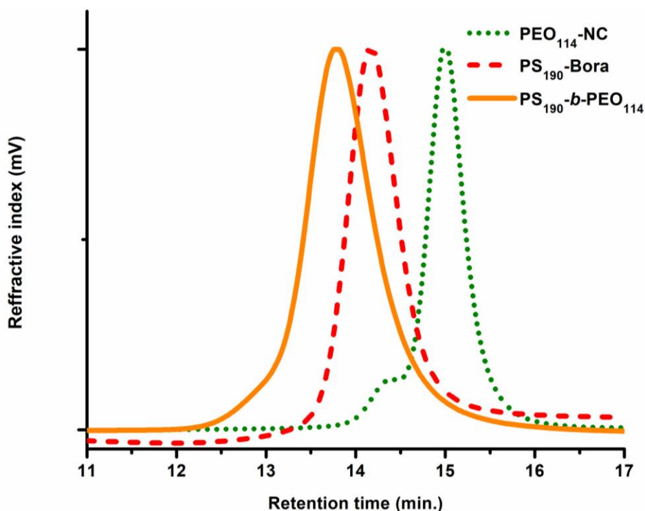
Figure 3. SEC traces of MeO-PEO 114 -NC, PS 190 -Bora and corresponding diblock copolymer PS 190 - b -PEO 114 in THF as the eluent.
