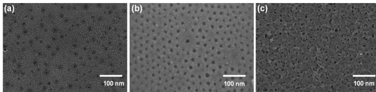
Figure 5. SEM micrographs of nanoporous polymeric material obtained from a) PS 167 - b -PEO 114 treated in ethanol, b) PS 167 - b -PEO 114 immersed in a TFA ethanol solution and c) PS 190 - b -PEO 114 treated in a TFA ethanol solution.
