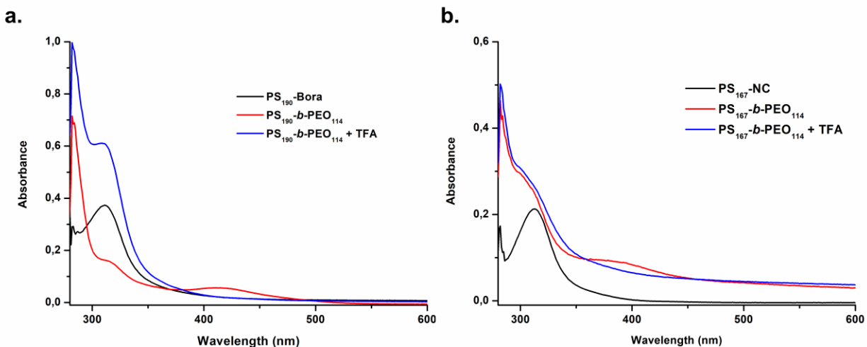
Figure 4. a. UV-vis spectra of PS 190 -Bora (black trace), resulting PS 190 - b -PEO 114 diblock copolymer (red trace) and same diblock copolymer in a TFA solution in toluene (blue trace). b. UV-vis spectra of PS 167 -NC (black trace), resulting PS 167 - b -PEO 114 diblock copolymer (red trace) and same diblock copolymer in a TFA solution in toluene (blue trace).
