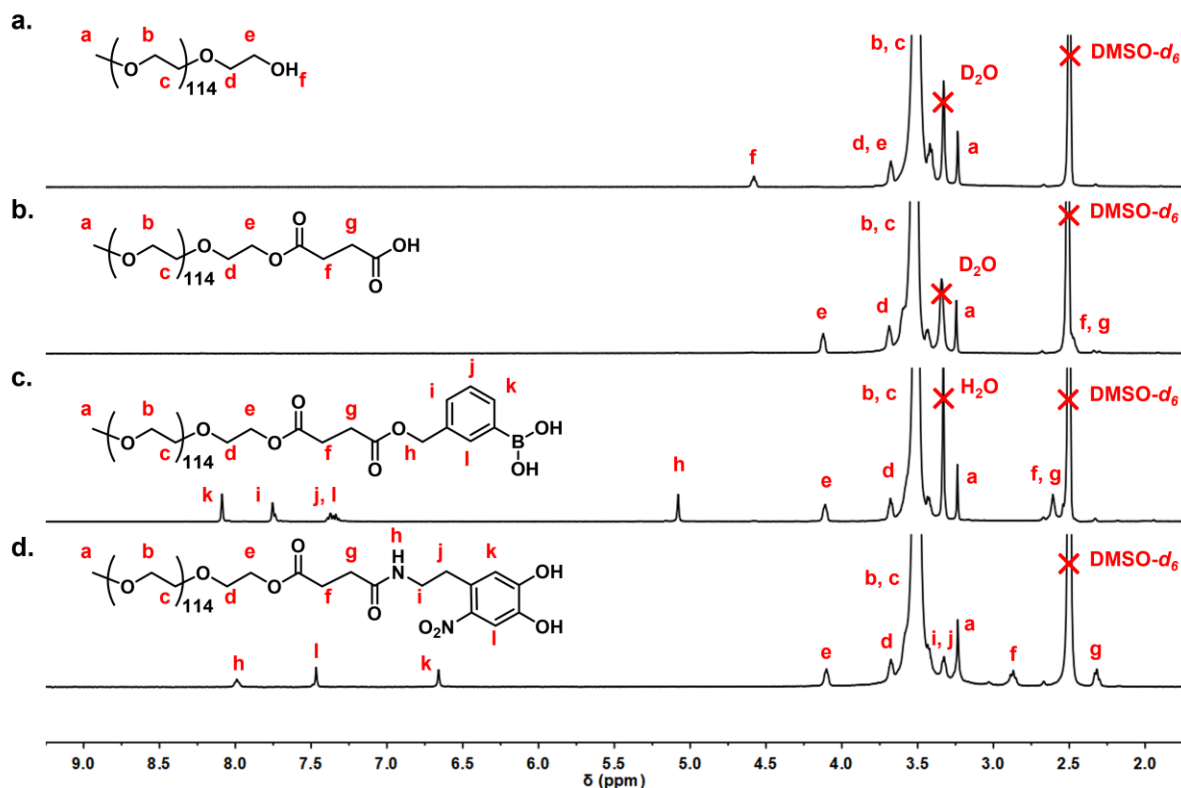
Figure 1. ^1\text{H} NMR spectra of: (a) MeO-PEO 114 -OH in D 2 O, (b) carboxylic acid end-functionalized PEO 114 (MeO-PEO 114 -COOH) in D 2 O, (c) boronic acid end-functionalized PEO 114 (MeO-PEO 114 -Bora) in DMSO- d 6 and (d) nitrocatechol end-functionalized PEO 114 (MeO-PEO 114 -NC) in DMSO- d 6 .
