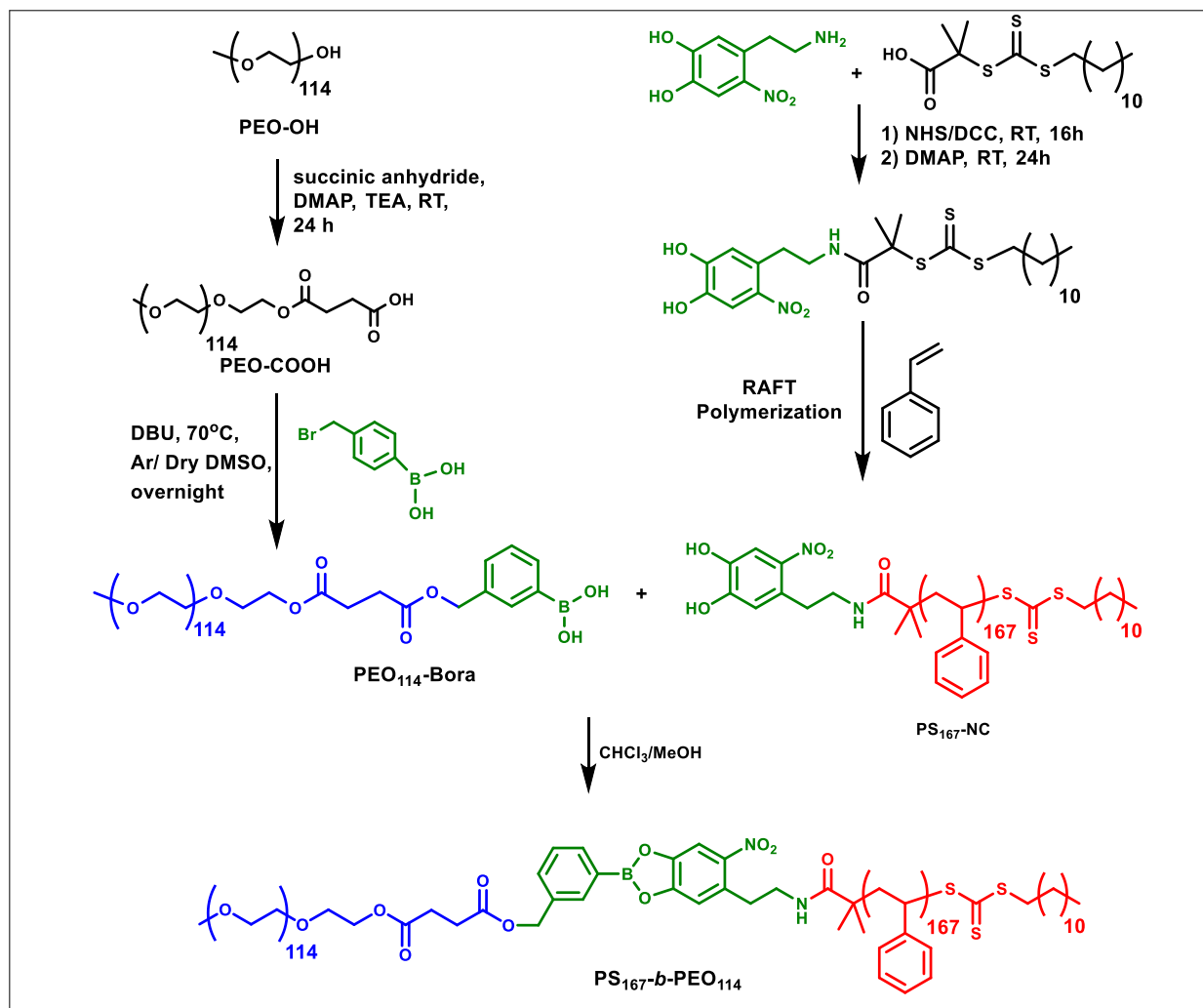
Scheme 1. Synthetic pathway towards boronate linked PS- b -PEO diblock copolymers by coupling reaction between nitrocatechol-ended PS and boronic acid-functionalized PEO homopolymers.
