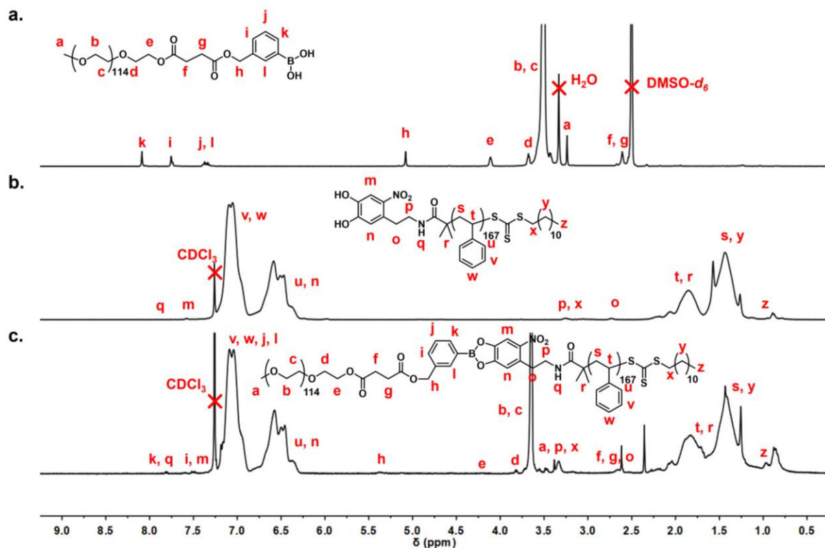
Figure 2. ^1\text{H} NMR spectra of (a) boronic acid end-functionalized poly(ethylene oxide) MeO-PEO 114 -Bora in DMSO- d 6 , (b) nitrocatechol end-functionalized polystyrene PS 167 -NC in CDCl 3 and (c) corresponding block copolymer PS 167 - b -PEO 114 in CDCl 3 .
