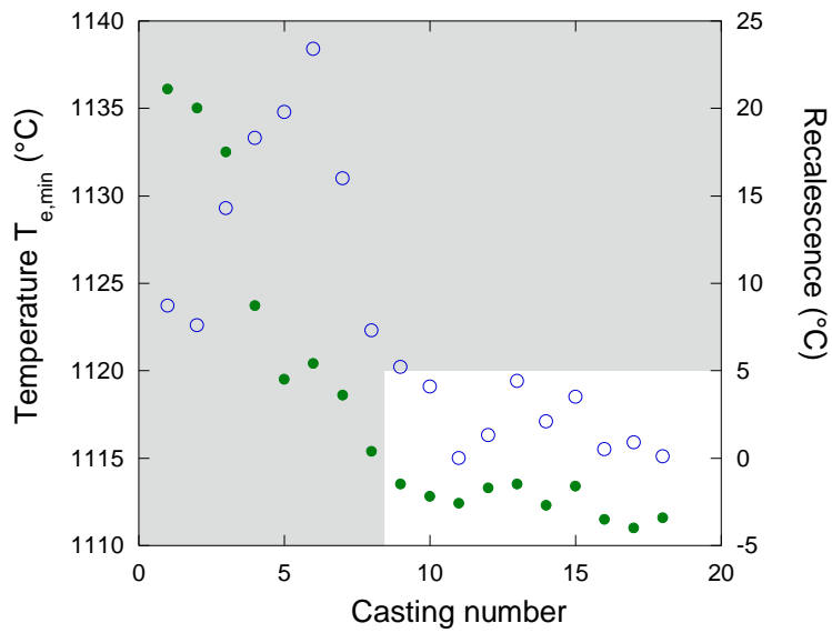
Figure B2. Plot of T_{e,min} (solid symbol) and recalescence (open symbols) for series 2.
