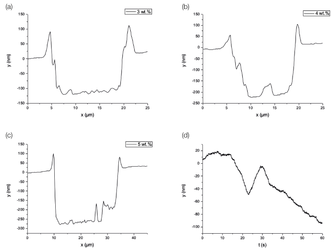
(a), (b) and (c) height profile from the AFM images shown above, force setpoint 500pN (d) height profile (profilometer scan in static mode 30μN), showing that PDMS has been deposited (tip is pushing down in static mode which corresponds to the elastomeric properties of PDMS).
