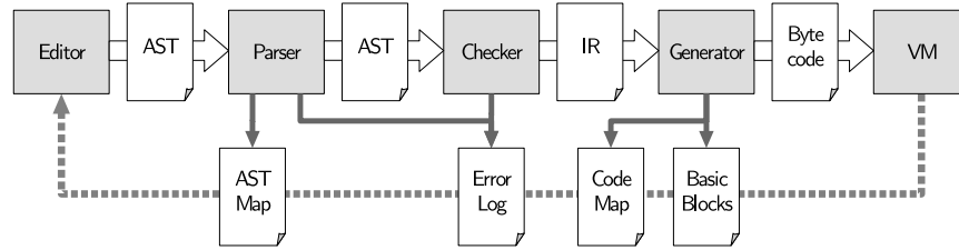
Figure 2. Quadrant Pipeline
