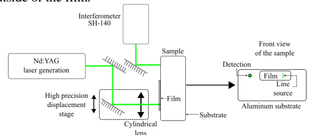
Figure 5 – Laser-ultrasonics setup.
