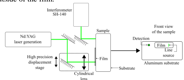
Figure 5 – Laser-ultrasonics setup.
