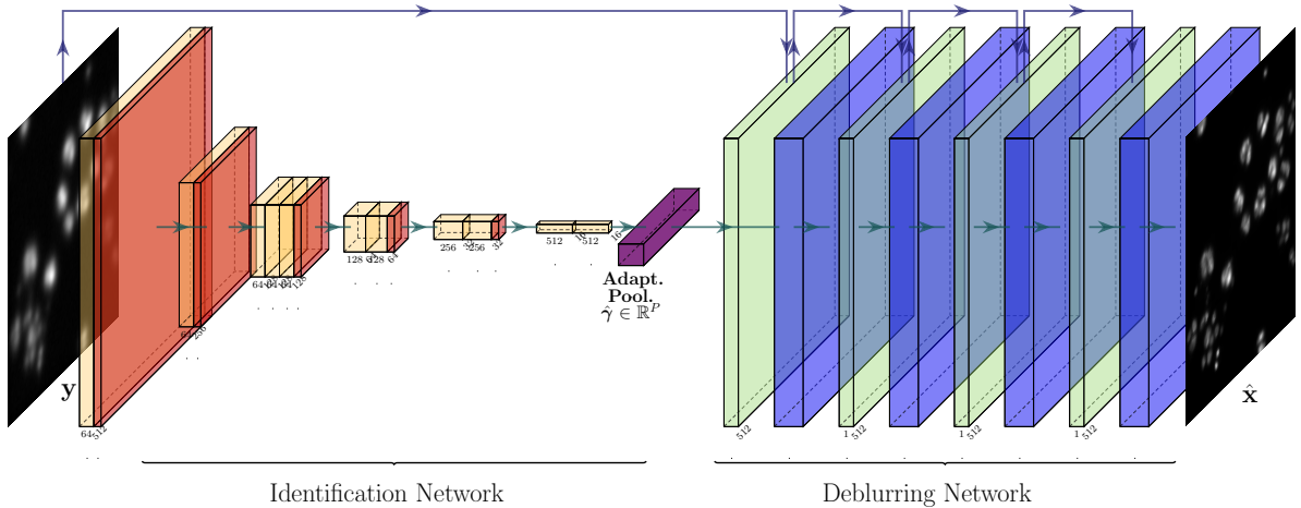
Figure 1: The Deep-Blur architecture. The first part of the network identifies the parameter \hat{\gamma} . In this paper, we use a ResNet architecture. The estimated parameter \hat{\gamma} is given as an input of a second deblurring network. This one is an unrolled Douglas-Rachford algorithm. The yellow blocks are convolution layers with ReLU and batch normalization. The red ones are average pooling layers. The green ones are regularized inverse layers of the form \mathbf{x}_{t+1} = (\mathbf{A}^*(\hat{\gamma})\mathbf{A}(\hat{\gamma}) + \lambda\mathbf{I})^{-1}\mathbf{A}(\hat{\gamma})\mathbf{y} . The violet blocks are U-Net like neural networks with weights learned to provide a sharp image \hat{\mathbf{x}}
