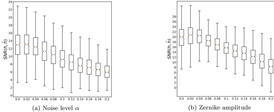
Figure 5: Stability of the kernel estimation with respect to noise level (left) and amplitude of the Zernike coefficients in the noiseless regime(right)
