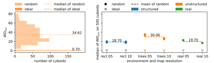
Fig. 2: Left: distribution of WD_{occ} on random and ideal reconstructions for an unstructured environment in simulation, on 500 cuboids, with the values of the medians. Right: summary of the medians of WD_{occ} on random and ideal reconstructions on all our environments. The dashed-lines are the limits for each environment ( WD_{occ}^* ).
