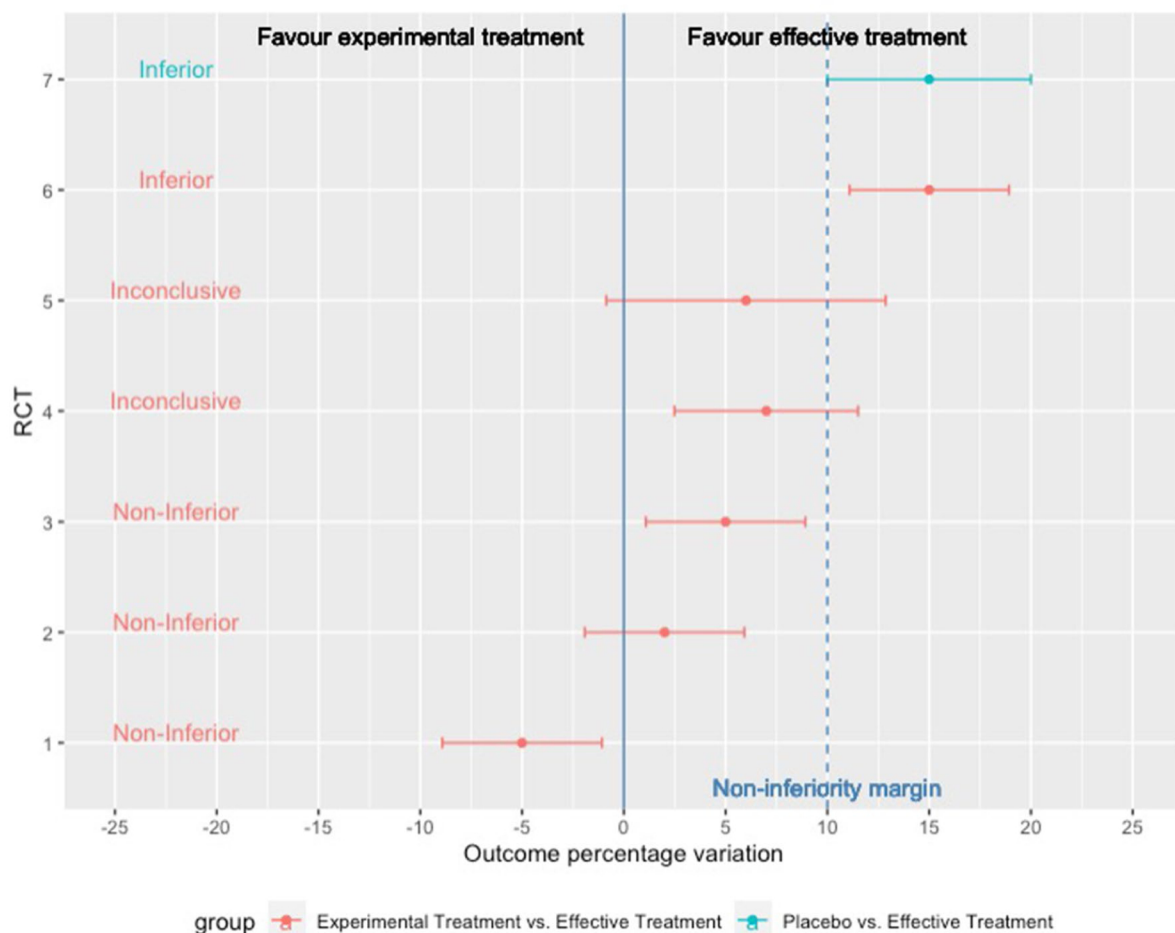
Fig. 1 Simulation of one superiority trial including the active control vs. placebo (RCT 7) and six non-inferiority RCTs (from 1 to 6) comparing the experimental treatment with the active control. The lower confidence interval boundary of the superiority trial defines the non-inferiority margin for the non-inferiority RCTs (dashed blue line). Three different scenarios can be identified concerning the non-inferiority query: non-inferiority, inconclusiveness, and inferiority. Besides RCT 7, in this example, we have not considered superiority issues in relation to the zero threshold (continuous blue line). Indeed, in trial 1 we also have superiority of the experimental treatment compared to the active control, while in trials 3, 4, and 6, it is inferior. RCT 3 is a particular, and mostly theoretical, case of non-inferiority in the non-inferiority perspective, and inferiority when adopting a superiority design (using the zero-difference threshold)
