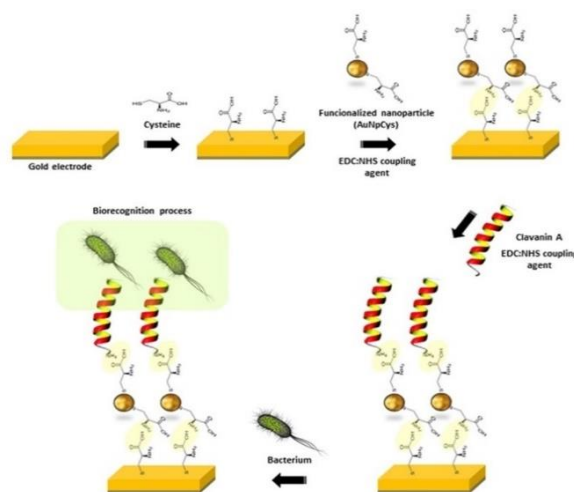
Fig. 3. Schematic representation on the functionalization steps including the cystein functionalization of gold electrode followed by the immobilization of functionalized gold-nanoparticles and then Clavanin A by coupling reactions. From De Miranda et al. [43], reprinted with permission.
