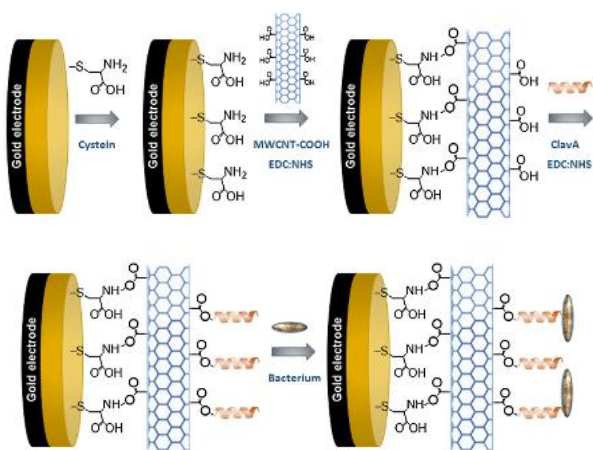
Fig. 10. Schematic representation of the nanostructured sensor based on carbon nanotubes: the peptide is bound on the CNTs surface and the interaction of the sensor with the bacteria is evaluated. From Andrade et al. [69], reprinted with permission.
