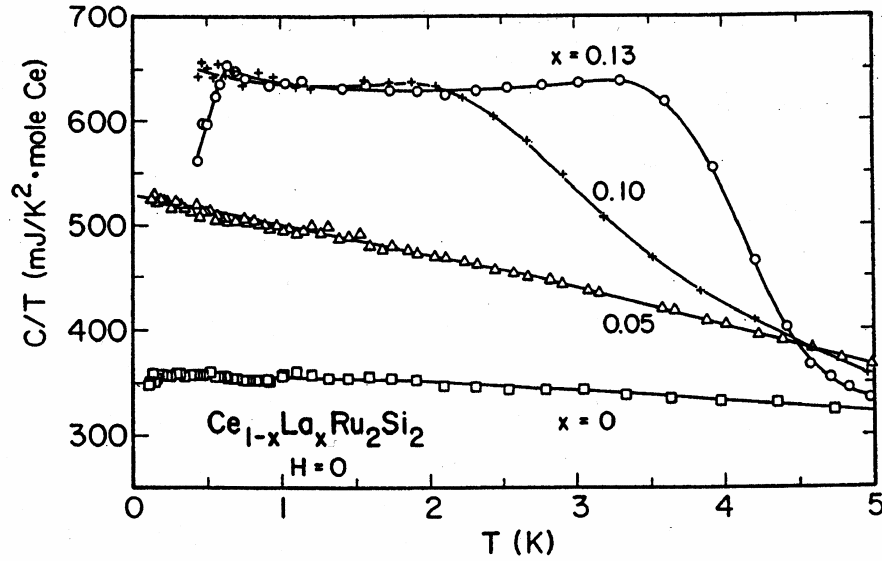
Fig. 4. Specific heat of Ce 1-x La x Ru 2 Si 2 on the both side of the critical concentration x_c = 0.075 .
