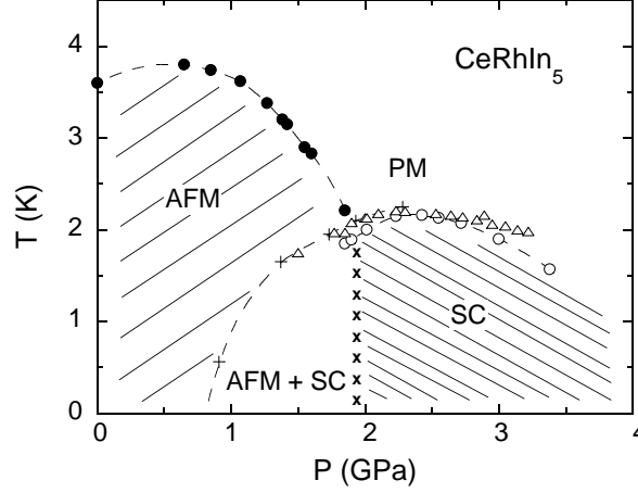
Fig. 7. Phase diagram of \text{CeRhIn}_5 as determined by specific heat ( \bullet and \circ ) and susceptibility ( \triangle ). In addition T_C(P) from resistivity measurements after, 45 ( \times ) marks the first order phase boundary between antiferromagnetism (AF) and superconductivity (SC).
