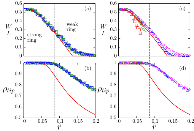
FIG. 2: MinE profile, characterized by W/L and \rho_{tip} , as a function of the scaled aspect ratio \tilde{r} . (a, b): Straight filaments ( p = \infty, \rho_0 = 0.35 ). 1D model results are shown with solid lines (using f = 0.06 ); 3D stochastic results are indicated by symbols. Single filaments ( n = 1 , green data) for L = 1 \mu\text{m} ( \square ), L = 2 \mu\text{m} ( \circ ) and L = 3 \mu\text{m} ( \triangle ); multiple filaments ( n = 2 , or 5 , blue data) for L = 1 \mu\text{m} ( \nabla ). (c, d): Helical filaments ( n = 1, \rho_0 = 0.35 ) with L/p = 20 ( \square , red), 10 ( \circ , green), 4 ( \triangle , blue) and 0 ( \diamond , pink). For all these data, \sigma_3 = 0.3 \mu\text{m}^3/s , and R is varied to explore \tilde{r} . Similar results are obtained when \sigma_3 is varied.
