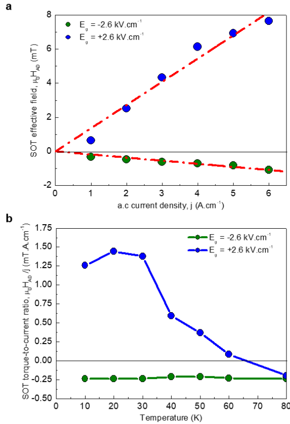
Figure 5 | Dependence of the spin-orbit torques anti-damping like components on the injected current density and on the temperature. a , Anti-damping like effective field \mu_0 H_{\text{AD}} as a function of the applied 2D current density for positive (blue) and negative (green) gate electric-field of \pm 2.6 \text{ kV} \cdot \text{cm}^{-1} at the temperature of 10K. Dashed and dotted lines are linear fits, yielding SOT effective fields \mu_0 H_{\text{AD}} = +1.36 \text{ mT} \cdot \text{A} \cdot \text{cm}^{-1} ( -0.18 \text{ mT} \cdot \text{A} \cdot \text{cm}^{-1} ) for positive (negative) gate electric-field. b , Temperature dependence of the SOT anti-damping like effective field \mu_0 H_{\text{AD}} at j = 2 \text{ A} \cdot \text{cm}^{-1} for positive (blue) and negative (green) gate electric-field of \pm 2.6 \text{ kV} \cdot \text{cm}^{-1} . All data have been measured with a nearly in-plane applied magnetic field ( \theta_H = 85^\circ , \phi_H = 45^\circ ).
